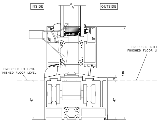
Open-in
